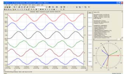
Real Time "Scope Mode" Waveforms and Phasor verification via PAS™
